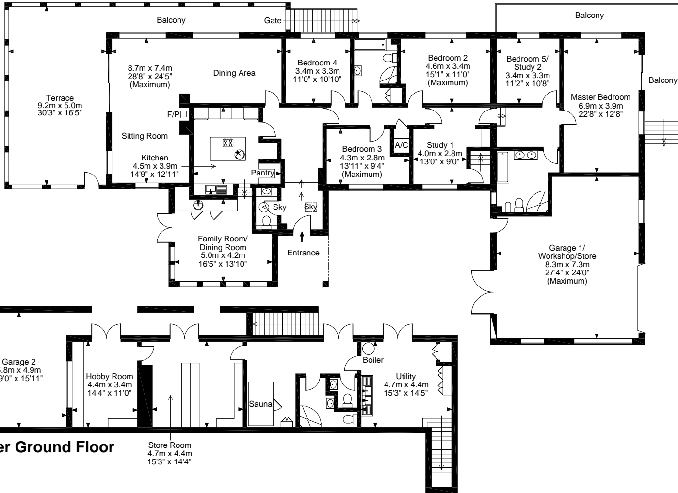
Green House
