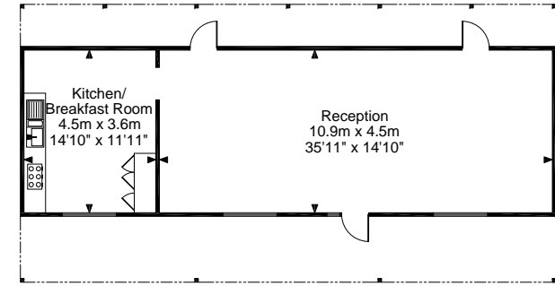
Lakeside Pavilion
